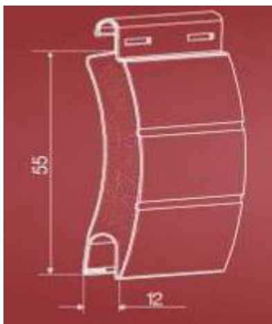
Stecche 12x55 mm
